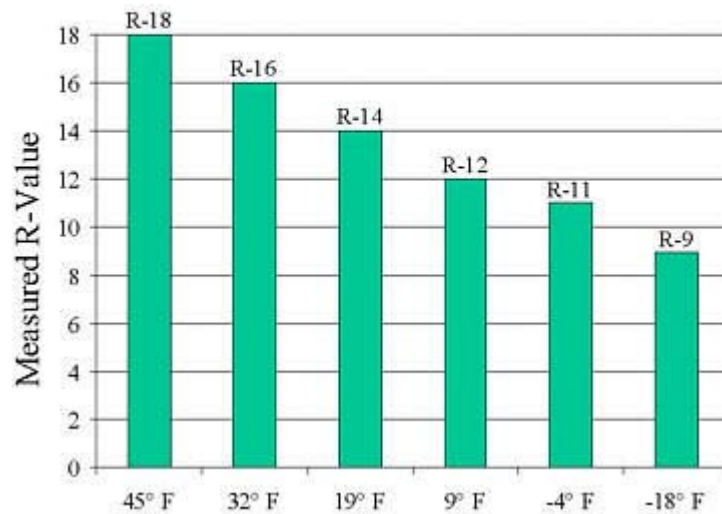
R-Value vs. Temperature For Loose-Fill Fiberglass
